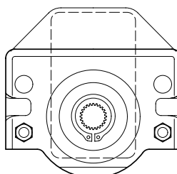
Side connection
